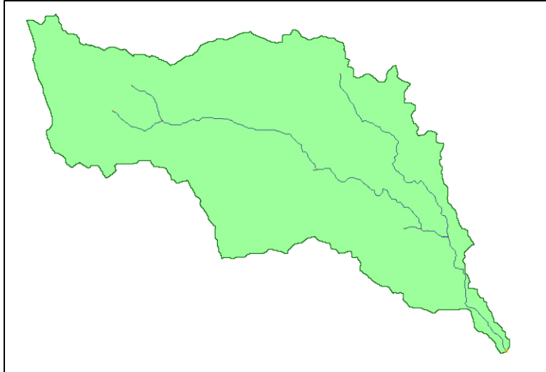
Figure 1 Delineated watershed
