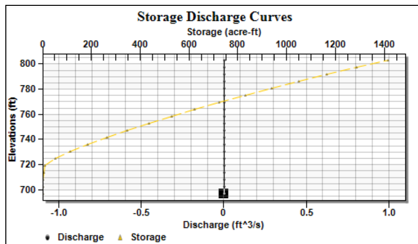
Figure 9 Storage discharge curve
