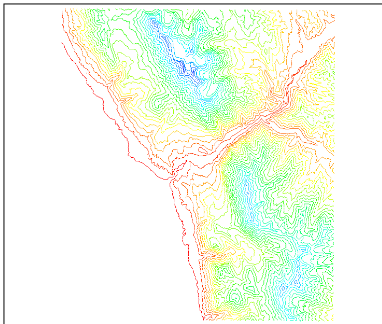
Figure 2-1 Starting project
